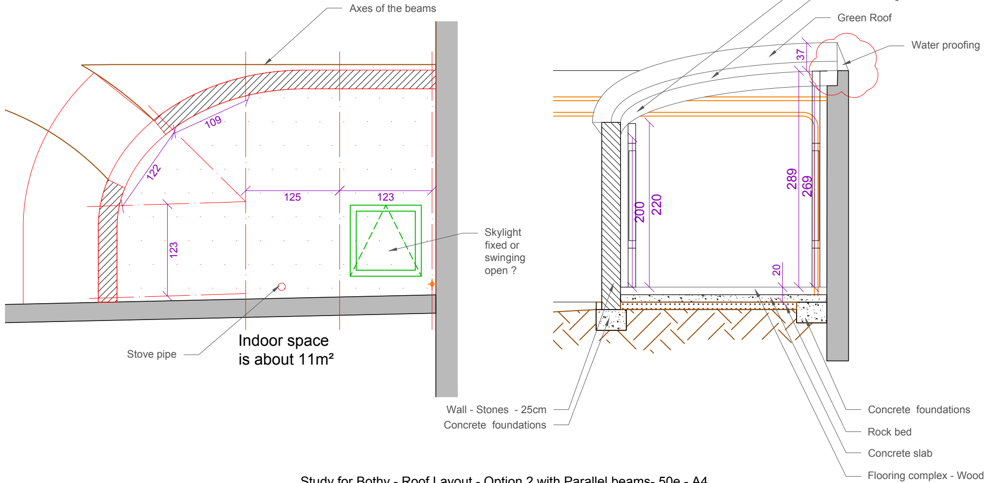
Study for Bothy - Roof Layout - Option 2 with Parallel beams- 50e - A4
