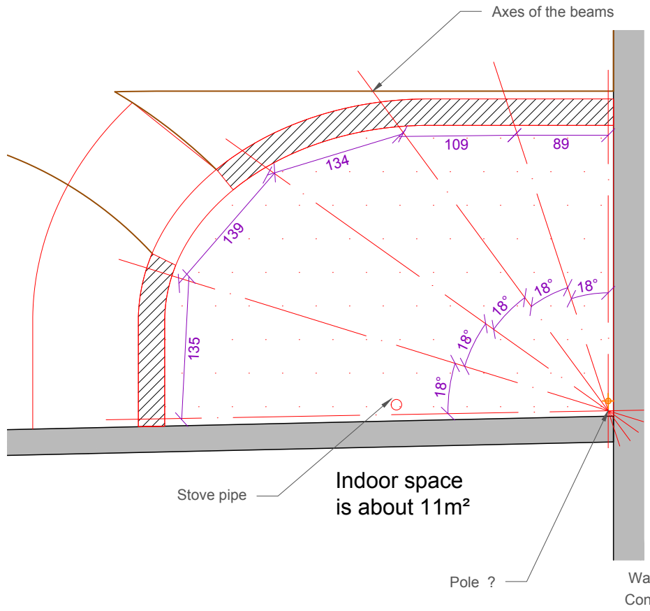
Study for Bothy - Roof Layout - Option 1 with a Pole - 50e - A4
