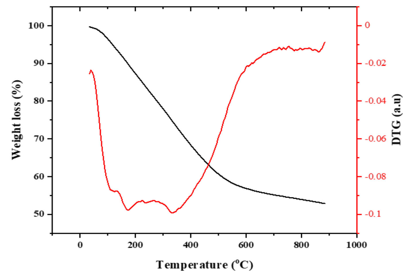
Figure 4 TGA/DTG thermograms of the raw alum sludge crumb showing three steps of major weight loss when heated up to 900°C.
