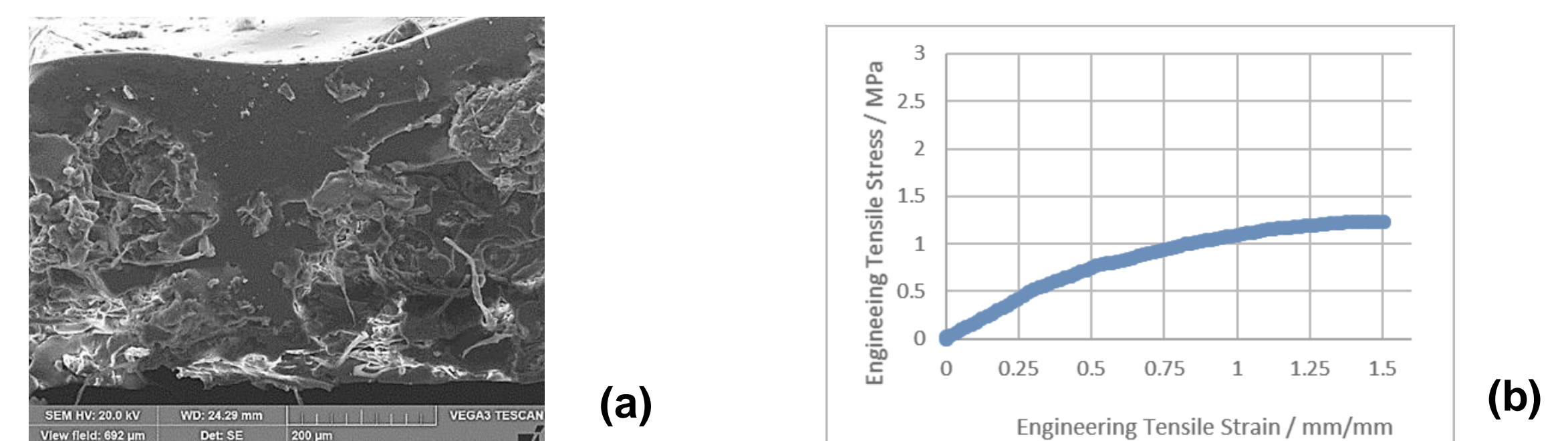
Figure 6 (a) SEM micrograph of composite cross-section and (b) its tensile test curve.
