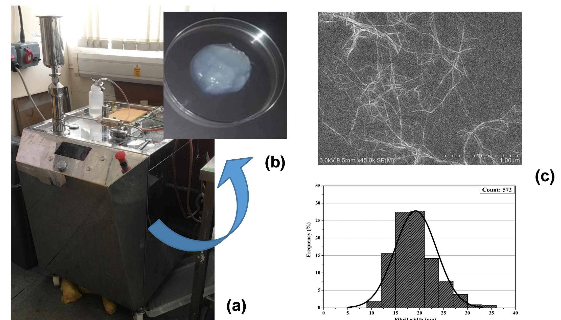
Figure 5 (a) the microfluidiser with 200 \mu\text{m} interaction chamber; (b) the processed CNF after 1pass in the chamber; (c) micrograph of CNF and their diameter size distribution.
