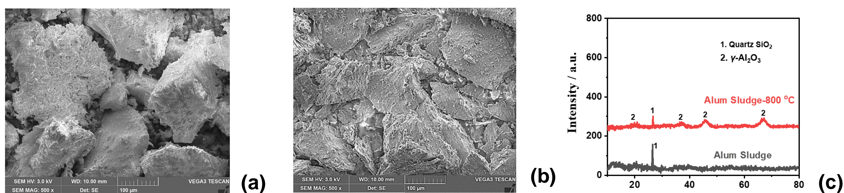
Figure 3 (a) FESEM images of untreated alum sludge crumb and (b) after being heat treated at 800°C; (c) XRD spectra for the raw and heat treated alum sludge.
